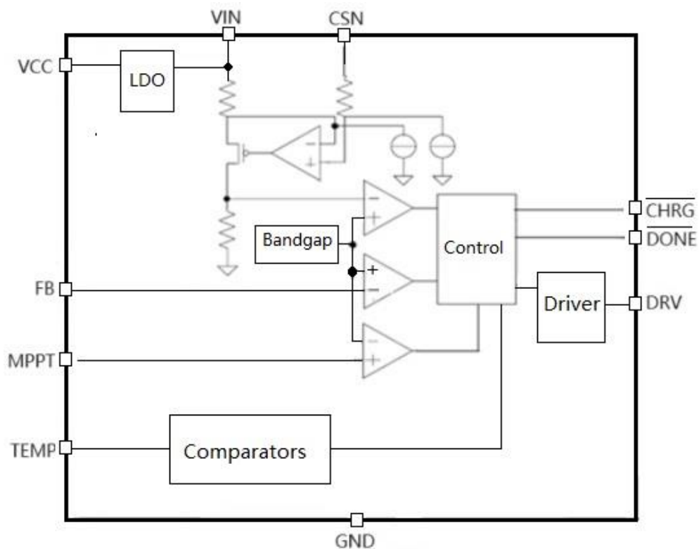
Figure 2 Block Diagram
