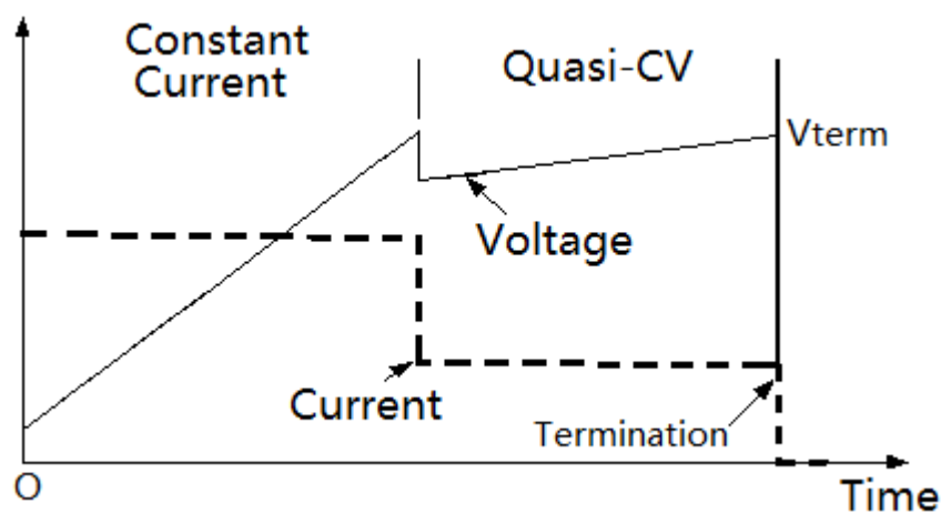
Figure 4 Charging Profile
